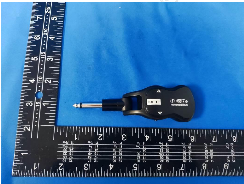
Photo 8 Overall view for receiver
